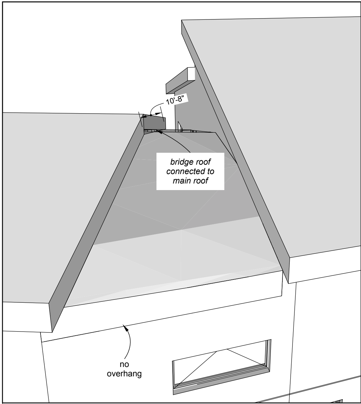
Detail: Bridge Roof from SW
